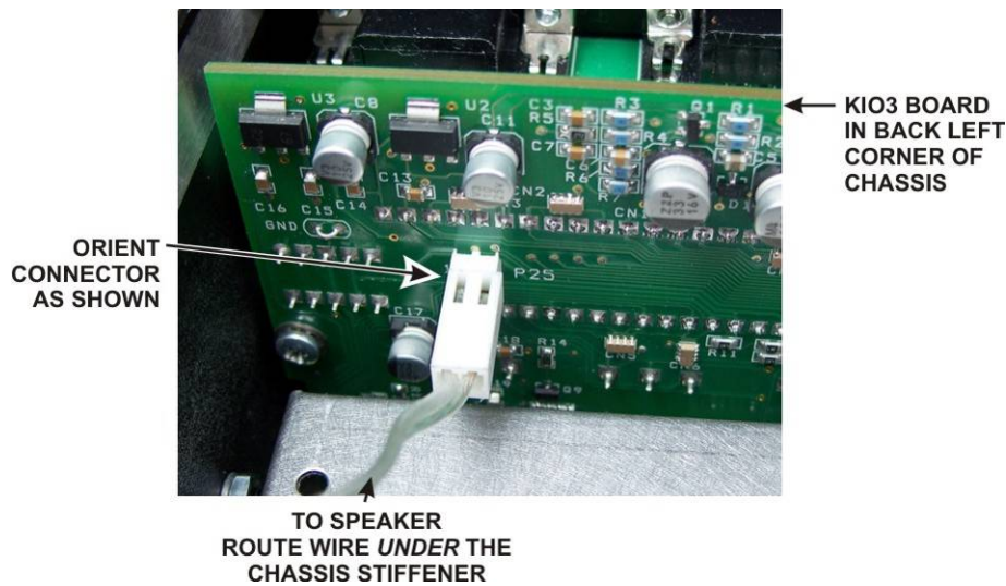
Figure 53. Connecting Speaker Cable.
