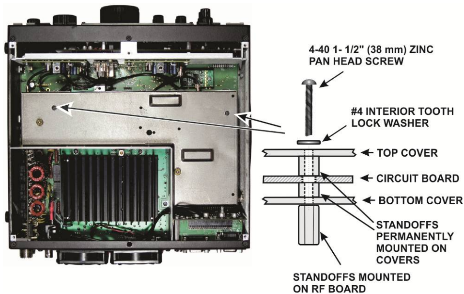
Figure 50. Installing the KRX3A Enclosure.
