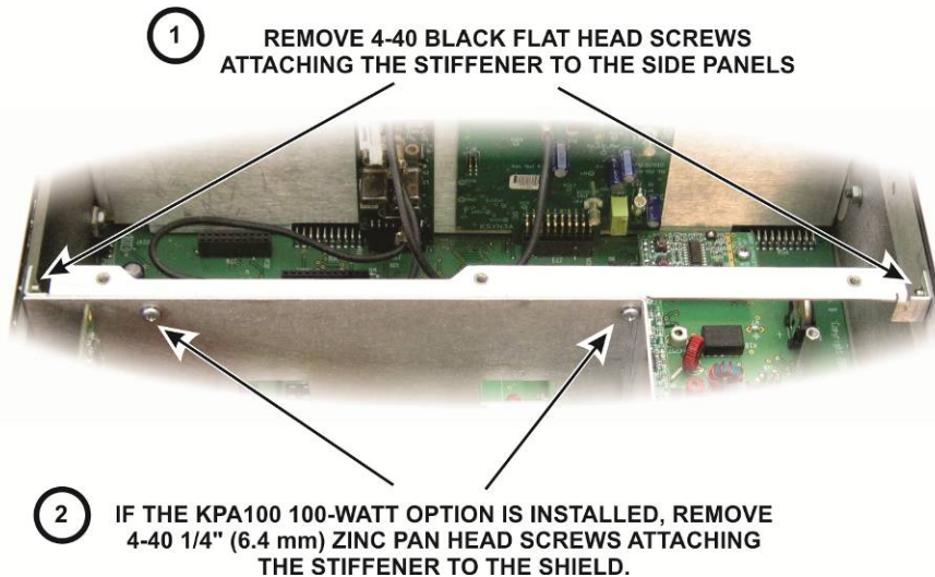
Figure 3. Removing the Chassis Stiffener Bar.
